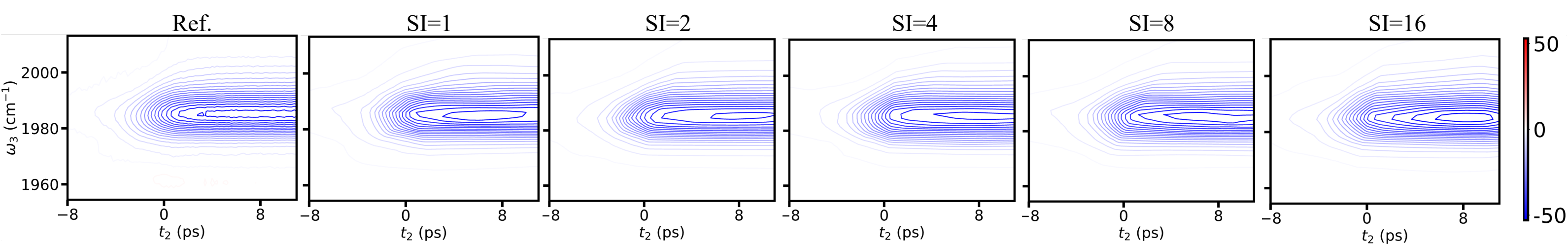
(a) Reference and recoveries from different sampling intervals (SI) on t_2
